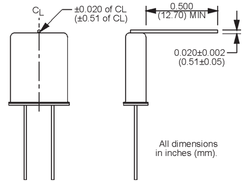
MP-1 with Ground Wire
