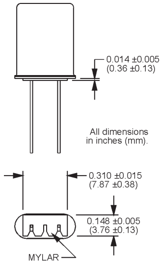
MP-1 with Insulator
